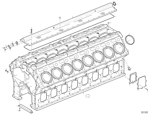
CRANKCASE UPC.06A01 2081
