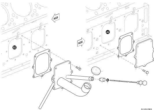
OIL FILLER NECK W OIL DIPSTICK, RGH XS595010.00074
